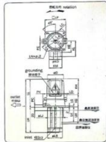
外型尺寸图 Externals dimensional drawing
