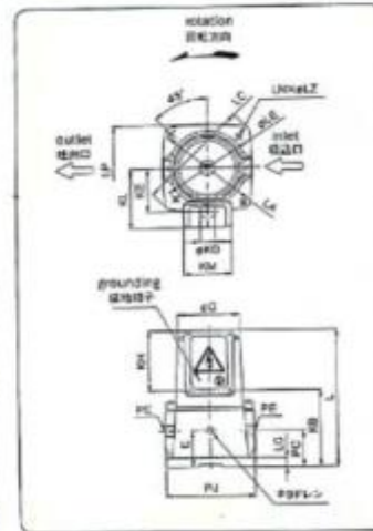
外型尺寸图 Externals dimensional drawing
