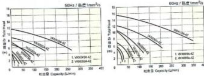
特性曲线 Characteristic curve
