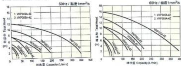
特性曲线 Characteristic curve
